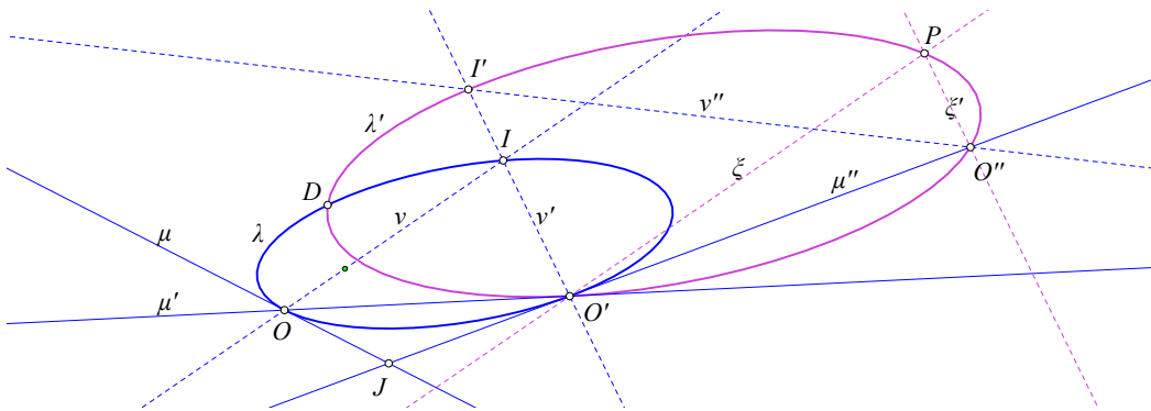
Figure 14: The image \lambda' = f(\lambda) of a conic of intersections is also a conic of intersections
